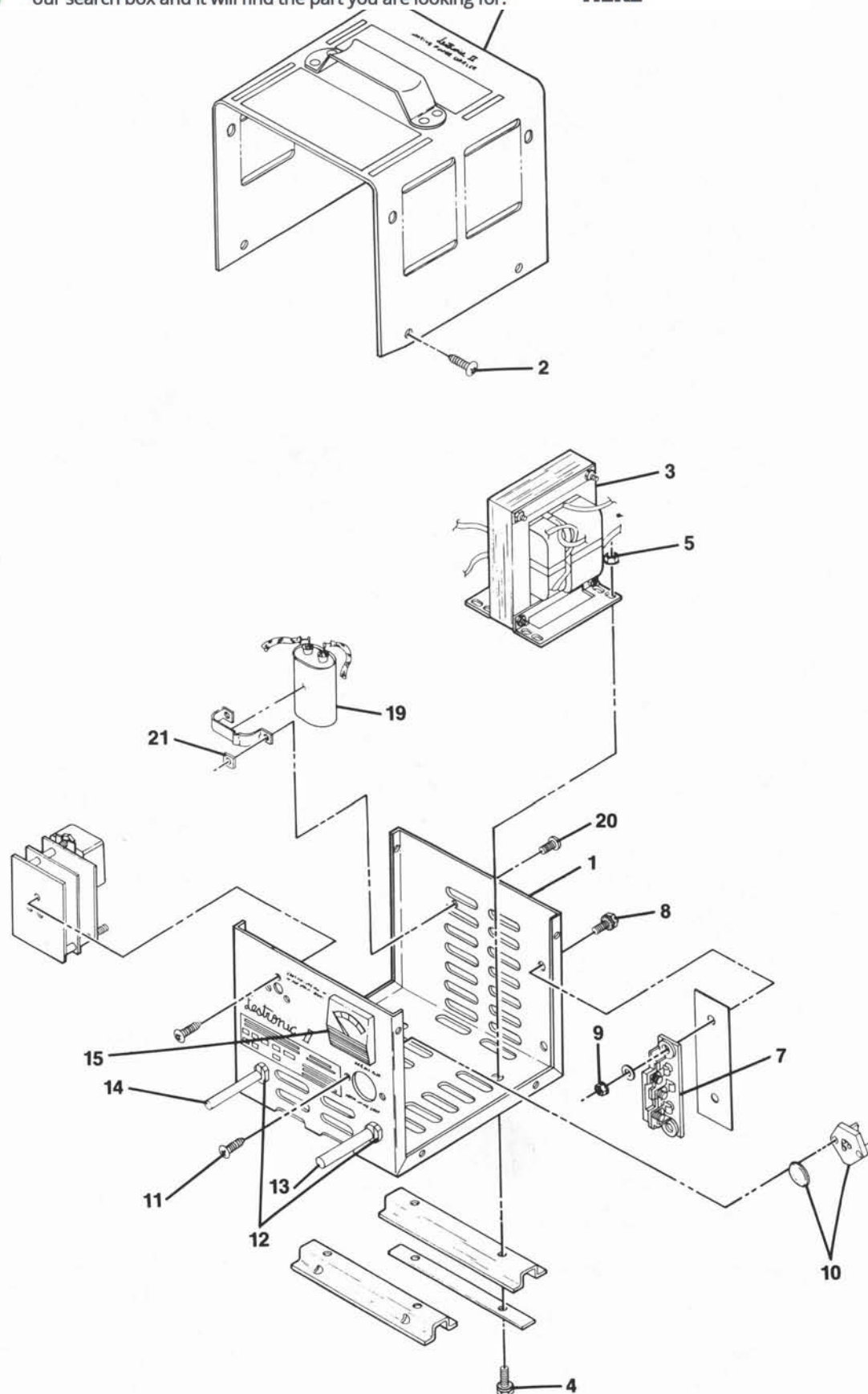
FIGURE 6-1. LESTER BATTERY CHARGER MODEL NO. 9611. SEE LIST 6-1.
