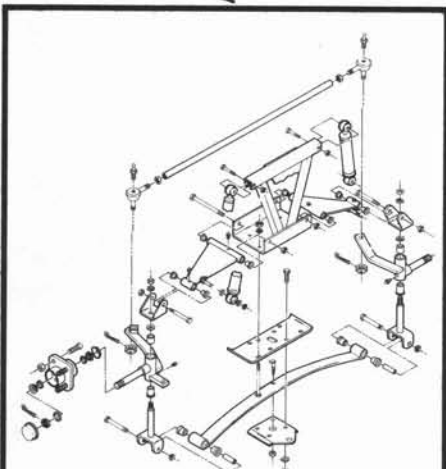
FRONT SUSPENSION ASS'Y FIGURE 2-3 PAGE 2-6
