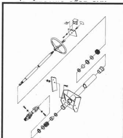
STEERING COLUMN ASS'Y FIGURE 2-1B PAGE 2-2B
