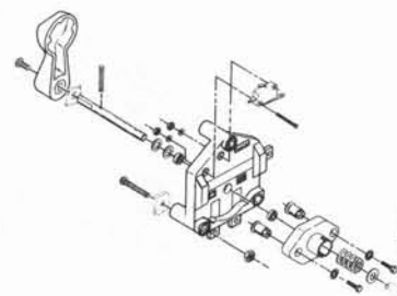
FORWARD & REVERSE SWITCH FIGURE 5-4 PAGE 5-8
