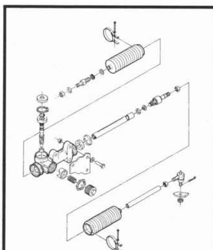
RACK & PINION ASS'Y FIGURE 2-2 PAGE 2-4
