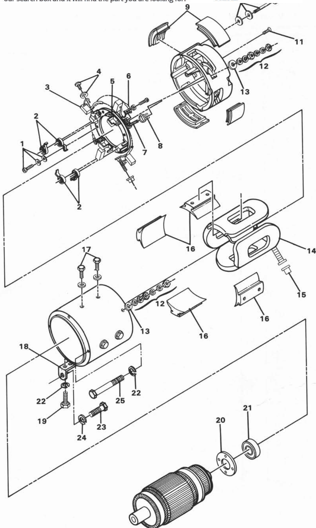
FIGURE 3-3. MOTOR ASSEMBLY FOR CLUB CAR MODEL 1012190. SEE LIST 3-3.
