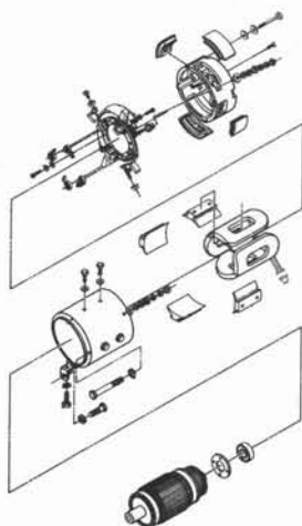
MOTOR ASS'Y FIGURE 3-2, PAGE 3-4 FIGURE 3-3, PAGE 3-6
