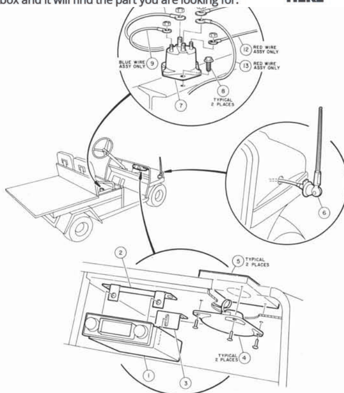
FIGURE 7-4. AM/FM STEREO RADIO. SEE LIST 7-4.
