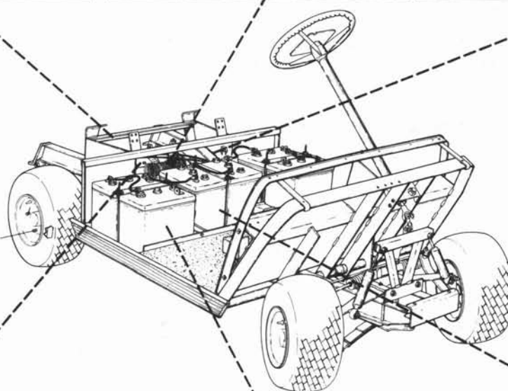
RESISTOR & BOARD ASS'Y FIGURE 5-3A PAGE 5-6A
