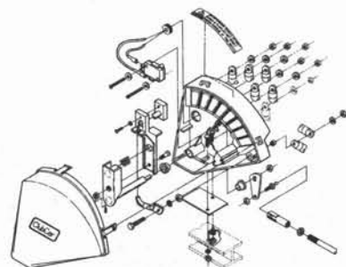
V-GLIDE ACCELERATOR SYSTEM FIGURE 5-2A PAGE 5-4A
