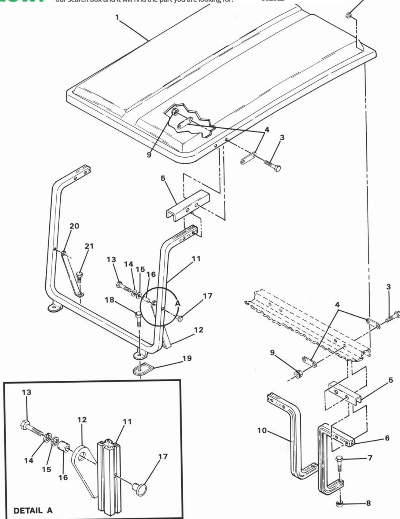
FIGURE 7-8. SPORTS CANOPY (STANDARD DS). SEE LIST 7-8.
