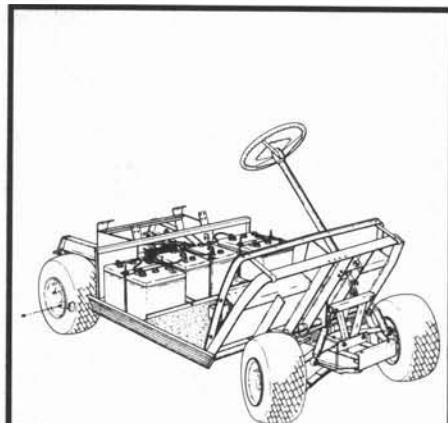
FINAL ASS'Y, ELECTRIC CAR FIGURE 1-1 (SHEET 2 OF 2) PAGE 1-4
