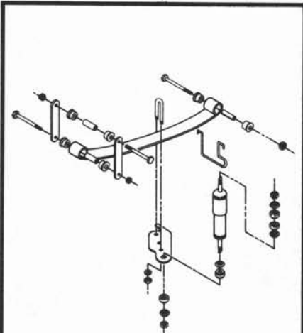
REAR SUSPENSION ASS'Y FIGURE 2-4A PAGE 2-8A
