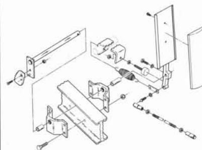
ACCELERATOR PEDAL ASS'Y FIGURE 4-3 PAGE 4-6
