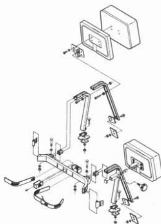
SEAT BACK & BAG HOOP ASS'Y FIGURE 1-4 PAGE 1-8
