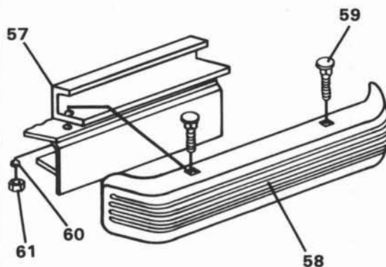
FIGURE 1-1A. FINAL ASSEMBLY, ELECTRIC CAR. SHEET 2 OF 2. INDEX NUMBERS 42-77. SEE LIST 1-1A.
