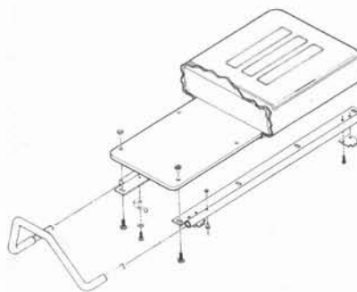
SEAT BOTTOM ASS'Y FIGURE 1-3 PAGE 1-7
