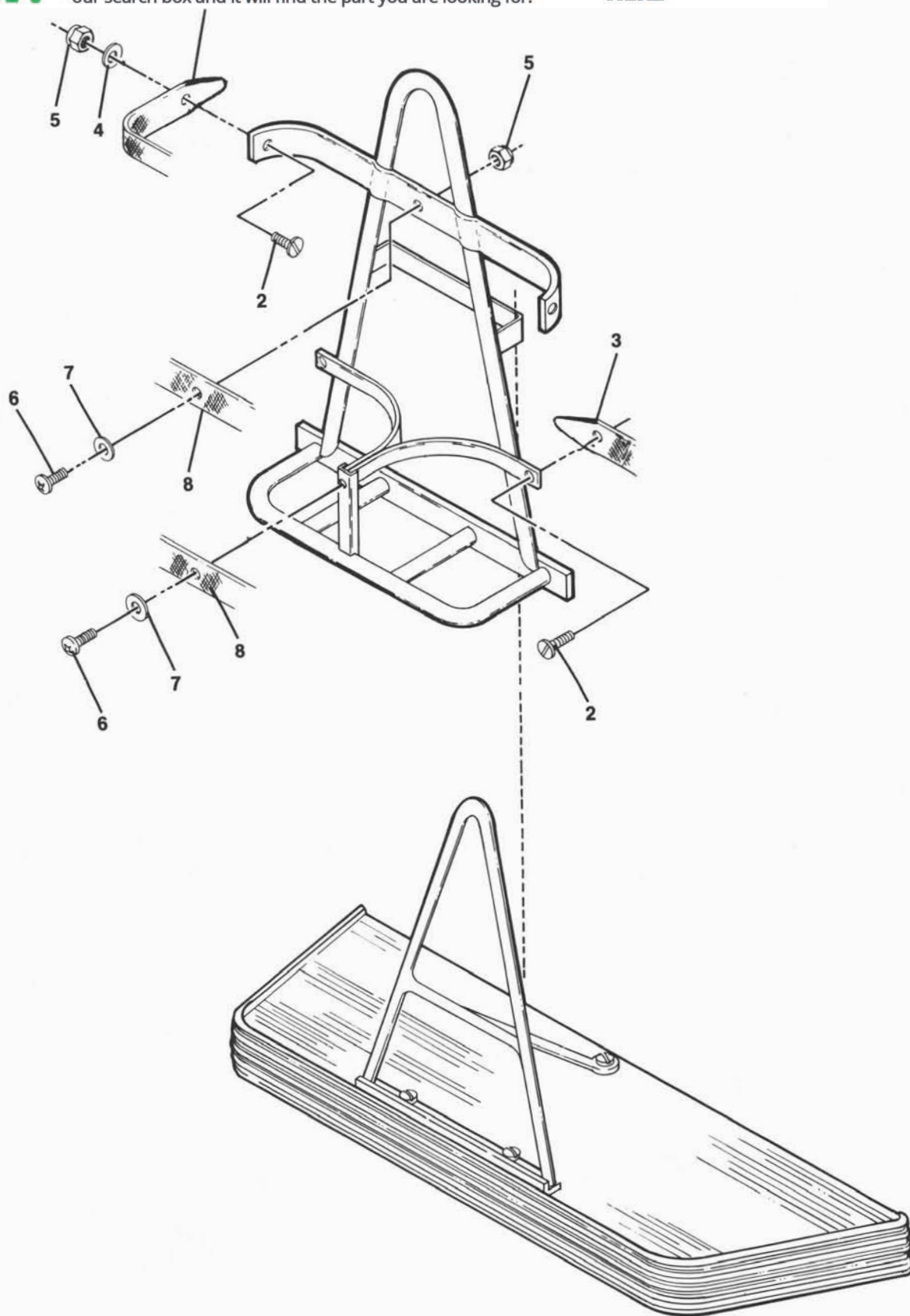
FIGURE 7-9. 2-BAG ATTACHMENT KIT (4-PASSENGER). SEE LIST 7-9.
