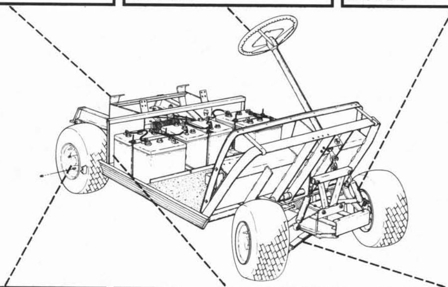
RACK & PINION ASS'Y FIGURE 2-2 PAGE 2-4
