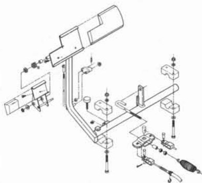
BRAKE PEDAL & CABLE ASS'Y FIGURE 4-2 PAGE 4-4
