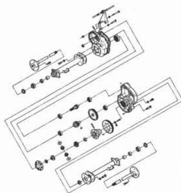
DRIVE UNIT FIGURE 3-1A PAGE 3-2A
