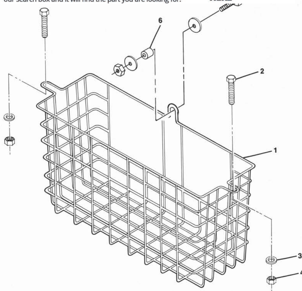
FIGURE 7-3. SWEATER BASKET. SEE LIST 7-3.
