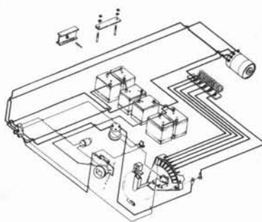
WIRING DIAGRAM FIGURE 5-1A PAGE 5-2A
