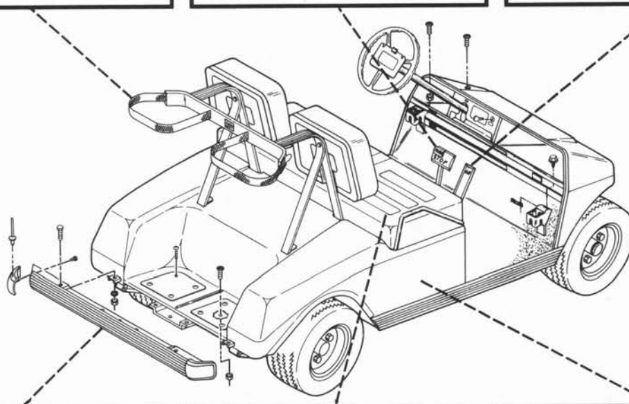
SEAT BACK & BAG HOOP ASS'Y FIGURE 1-4 PAGE 1-8
