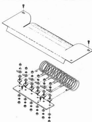
RESISTOR & BOARD ASS'Y FIGURE 5-3A PAGE 5-6A
