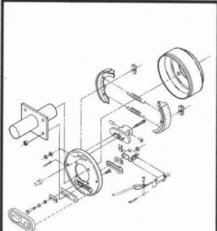
BRAKE CLUSTER, RIGHT & LEFT FIGURE 4-1 PAGE 4-2
