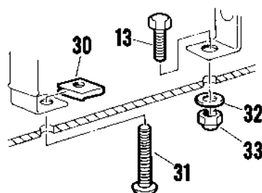
FIGURE 2-12C. FUEL SYSTEM ASSEMBLY. SEE LIST 2-12C.
