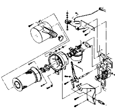
AIR CLEANER WITH CARBURETOR AND LINKAGE FIGURE 2-5 PAGE 2-12
