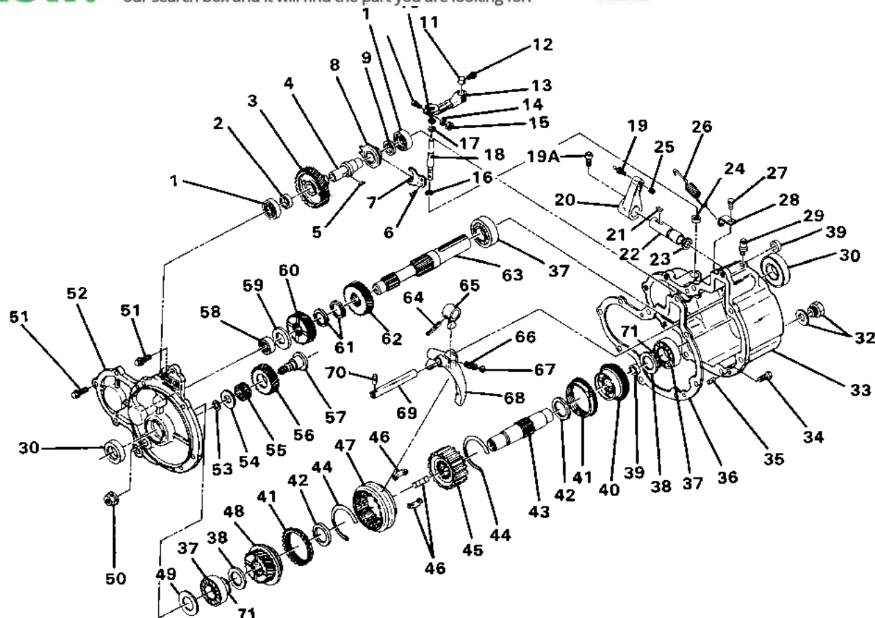
FIGURE 2-8. TRANSMISSION ASSEMBLY. SEE LIST 2-8.
