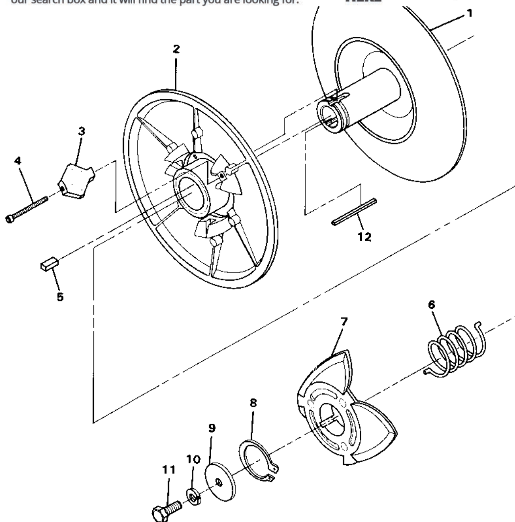
FIGURE 2-3A. DRIVEN CLUTCH. SEE LIST 2-3A.
