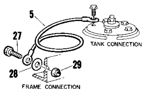
FIGURE 2-12C. FUEL SYSTEM ASSEMBLY. SEE LIST 2-12C.
