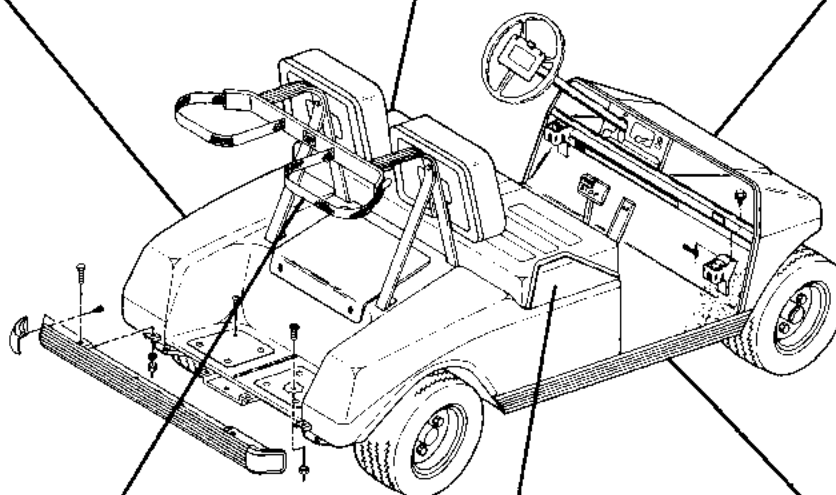
FINAL ASS'Y, GAS CAR FIGURE 1-1 (SHEET 1 OF 2) PAGE 1-2
