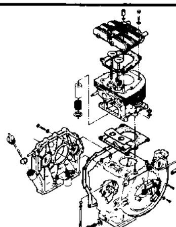
FINAL ASS'Y, ENGINE FIGURE 2-1 PAGE 2-4
