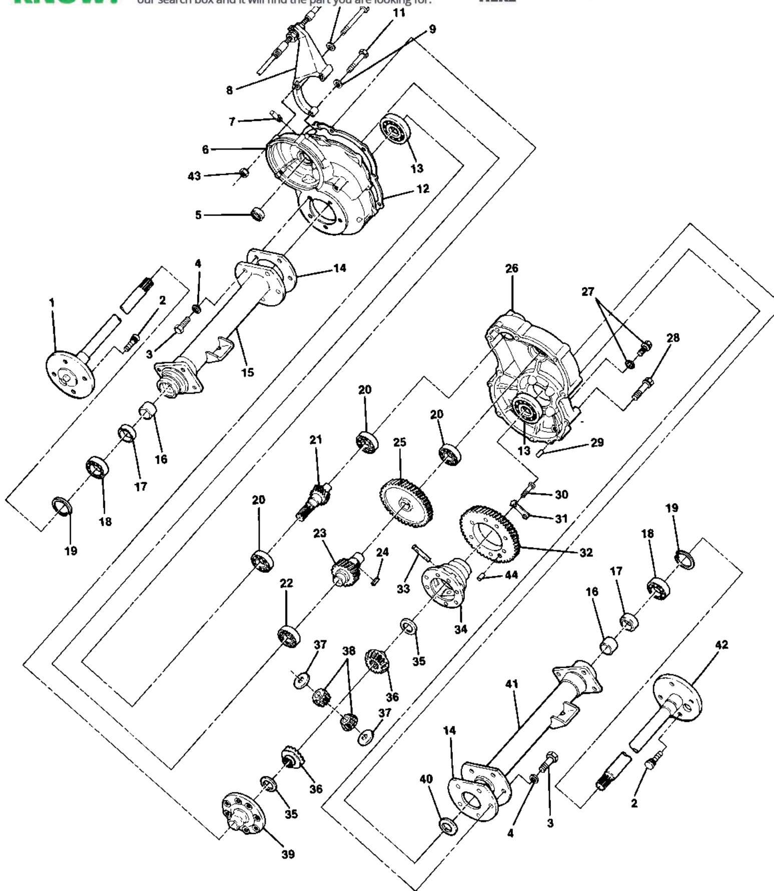
FIGURE 2-9. DRIVE UNIT. SEE LIST 2-9.
