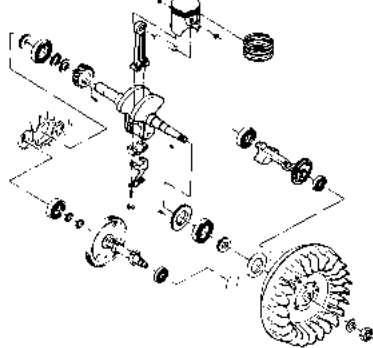
FINAL ASS'Y, ENGINE FIGURE 2-1 PAGE 2-6
