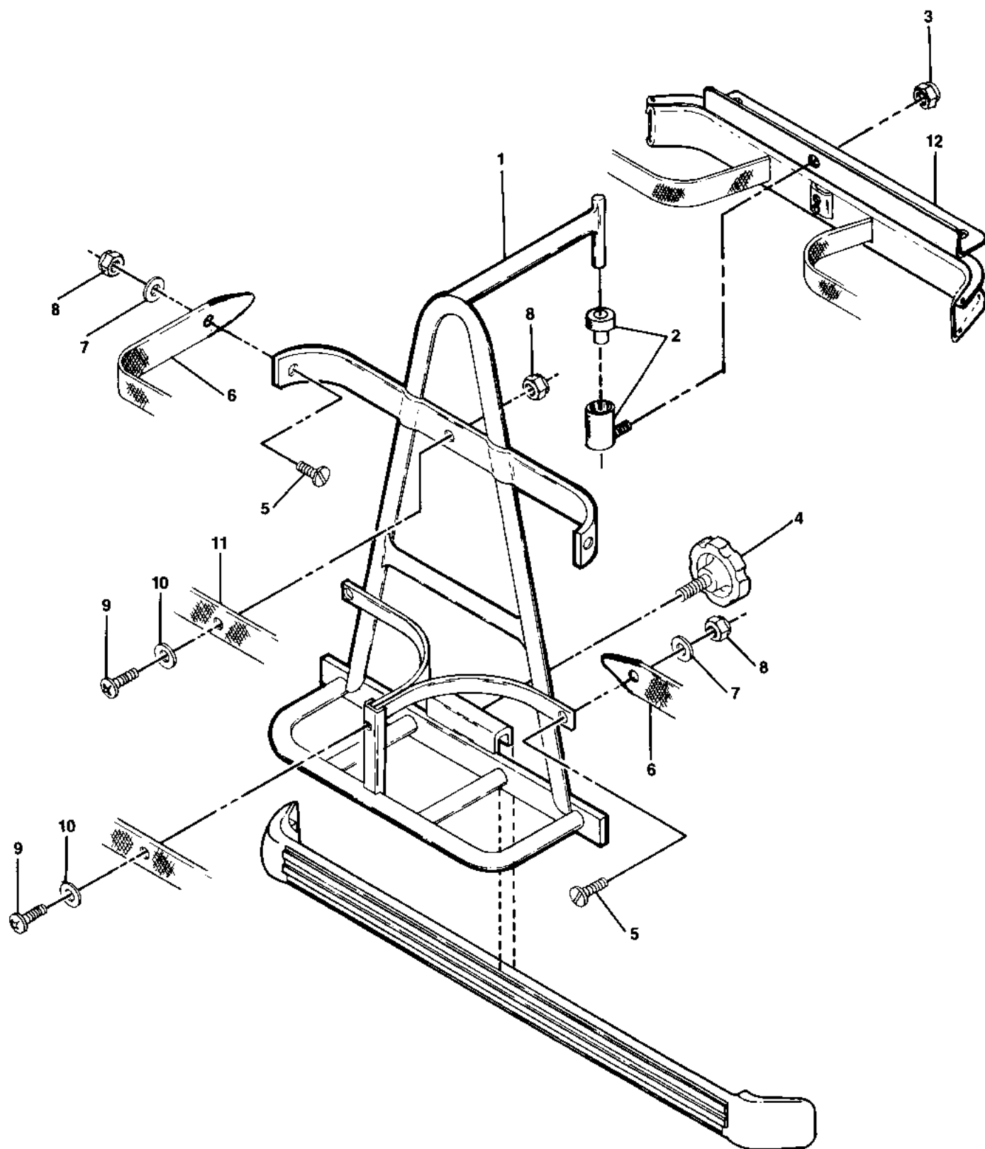
FIGURE 6-10. 4-BAG ATTACHMENT KIT (2-PASSENGER). SEE LIST 6-10.
