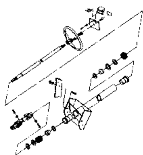
STEERING COLUMN ASS'Y FIGURE 3-1A PAGE 3-2A
