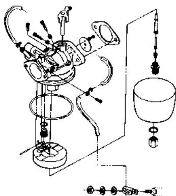
CARBURETOR ASS'Y FIGURE 2-6 PAGE 2-14
