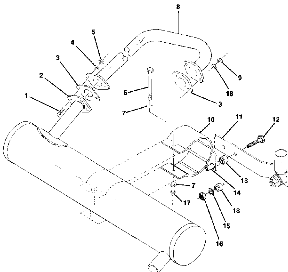
FIGURE 2-4. MUFFLER ASSEMBLY. SEE LIST 2-4.
