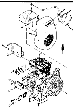
FINAL ASS'Y, ENGINE FIGURE 2-1 PAGE 2-2
