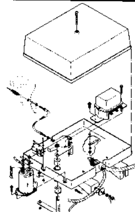
ELECTRICAL COMPONENT BOX ASSEMBLY FIGURE 5-2 PAGE 5-4
