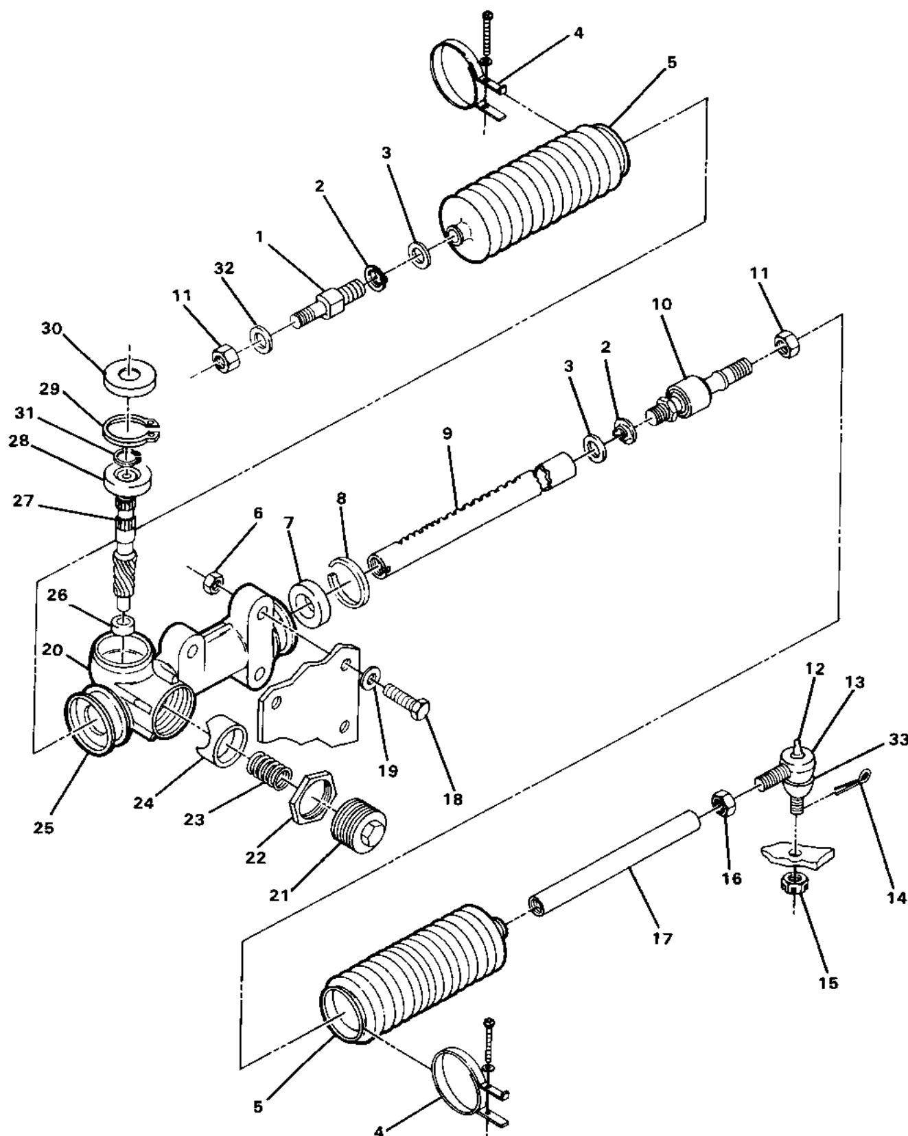
FIGURE 3-1. STEERING ASSEMBLY. SEE LIST 3-1.
