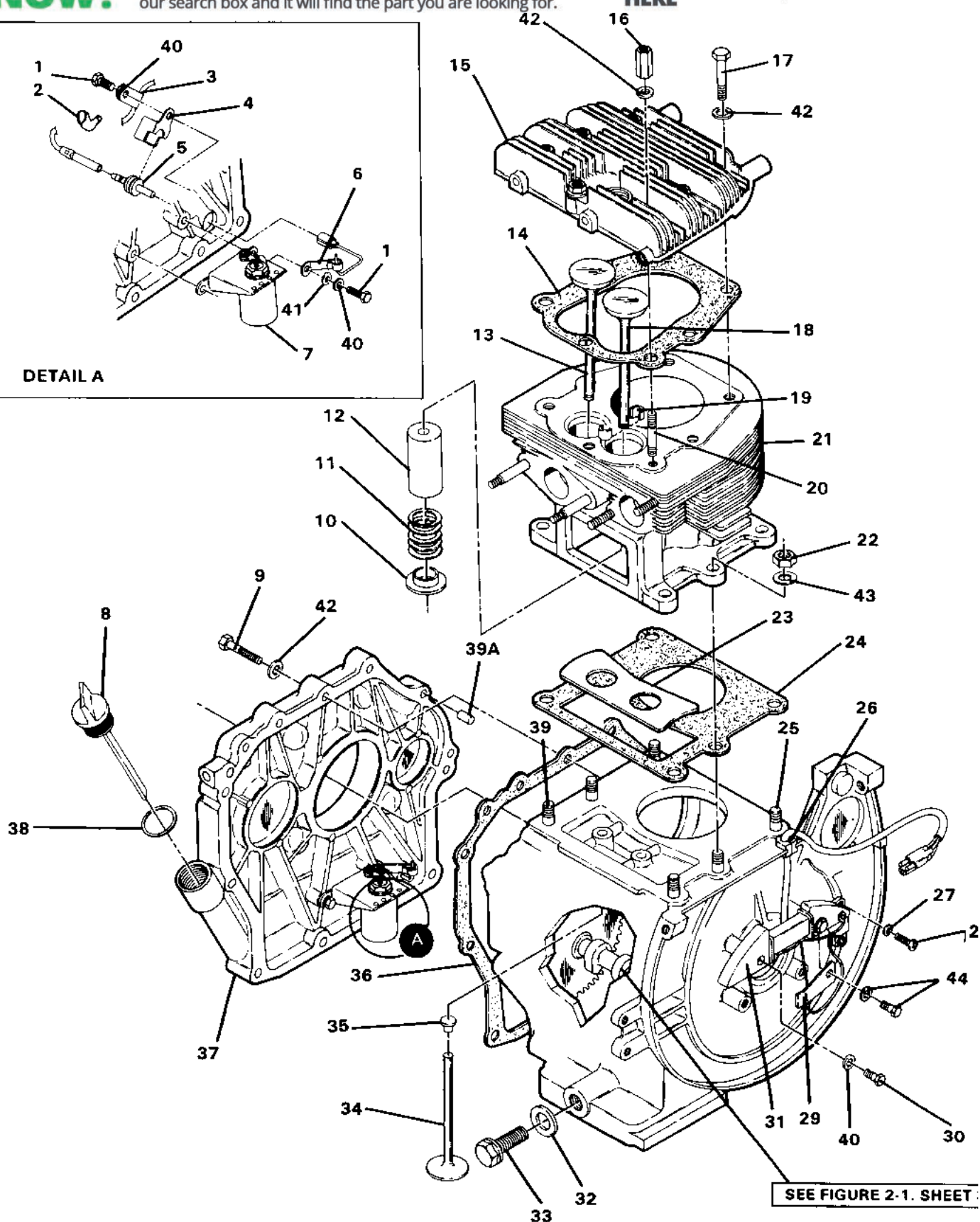
FIGURE 2-1. FINAL ASSEMBLY, ENGINE. SEE LIST 2-1.
