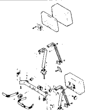
SEAT BACK & BAG HOOP ASS'Y FIGURE 1-3 PAGE 1-8
