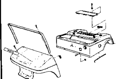
BODY ASS'Y, COVERS FIGURE 1-2 PAGE 1-6
