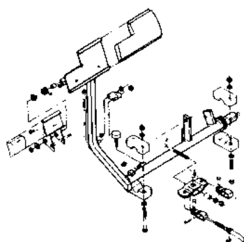
BRAKE PEDAL AND CABLE ASSEMBLY FIGURE 4-2 PAGE 4-4
