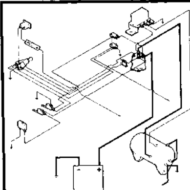
FINAL ASS'Y, WIRING DIAGRAM FIGURE 5-1 PAGE 5-2
