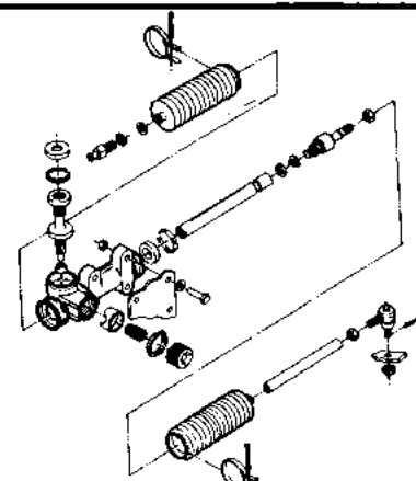
STEERING ASSEMBLY FIGURE 3-1 PAGE 3-4
