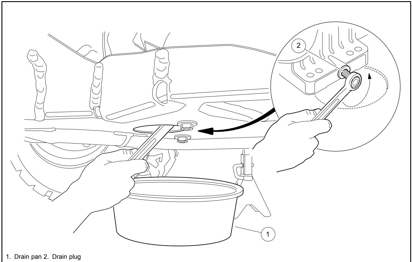
2667 Figure 34 Engine Oil Drain Plug and Pan
