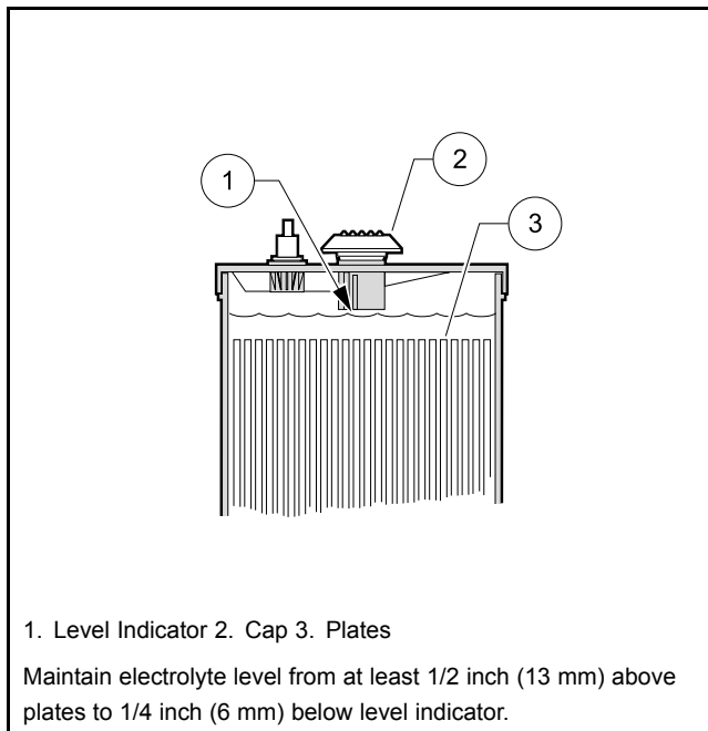
Figure 22 Electric Battery Electrolyte Level
