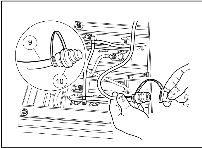
Figure 25 Dust Cap
