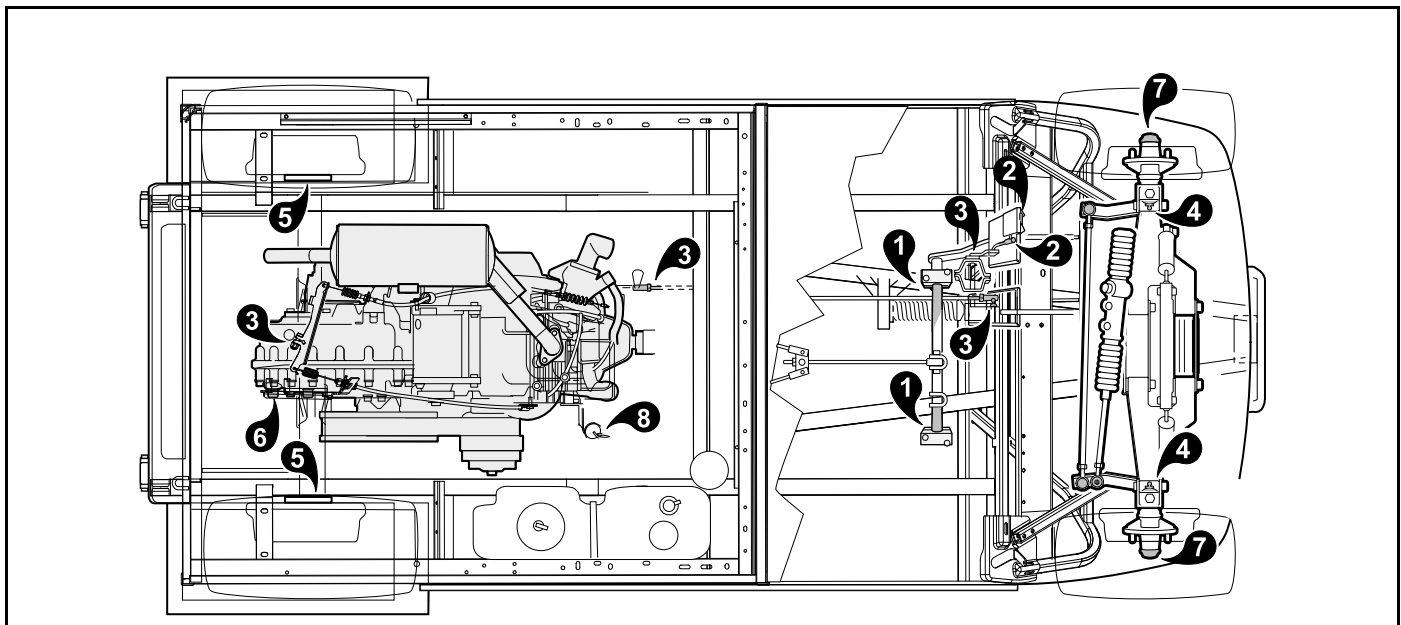
2778 Figure 21 Lubrication Points – Gasoline Vehicles
