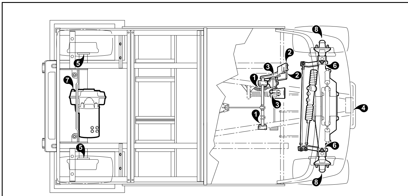
2777 Figure 20 Lubrication Points – Electric Vehicles
