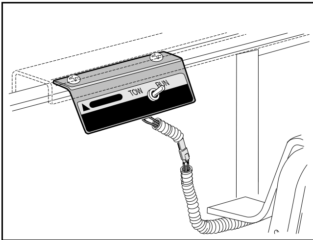
Figure 16 Tow/Run Switch
