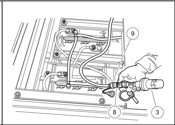
Figure 26 Connecting Hose-end Assembly to Battery Fill Connector
