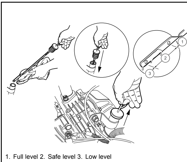
Figure 33 Engine Oil Level Check
