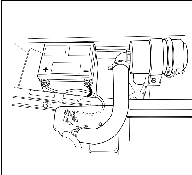
Figure 31 Gasoline Vehicle Battery
